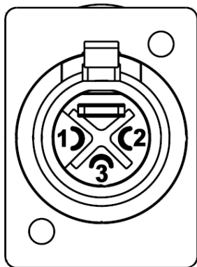
XLR PINS BACK SIDE PANEL JACK
